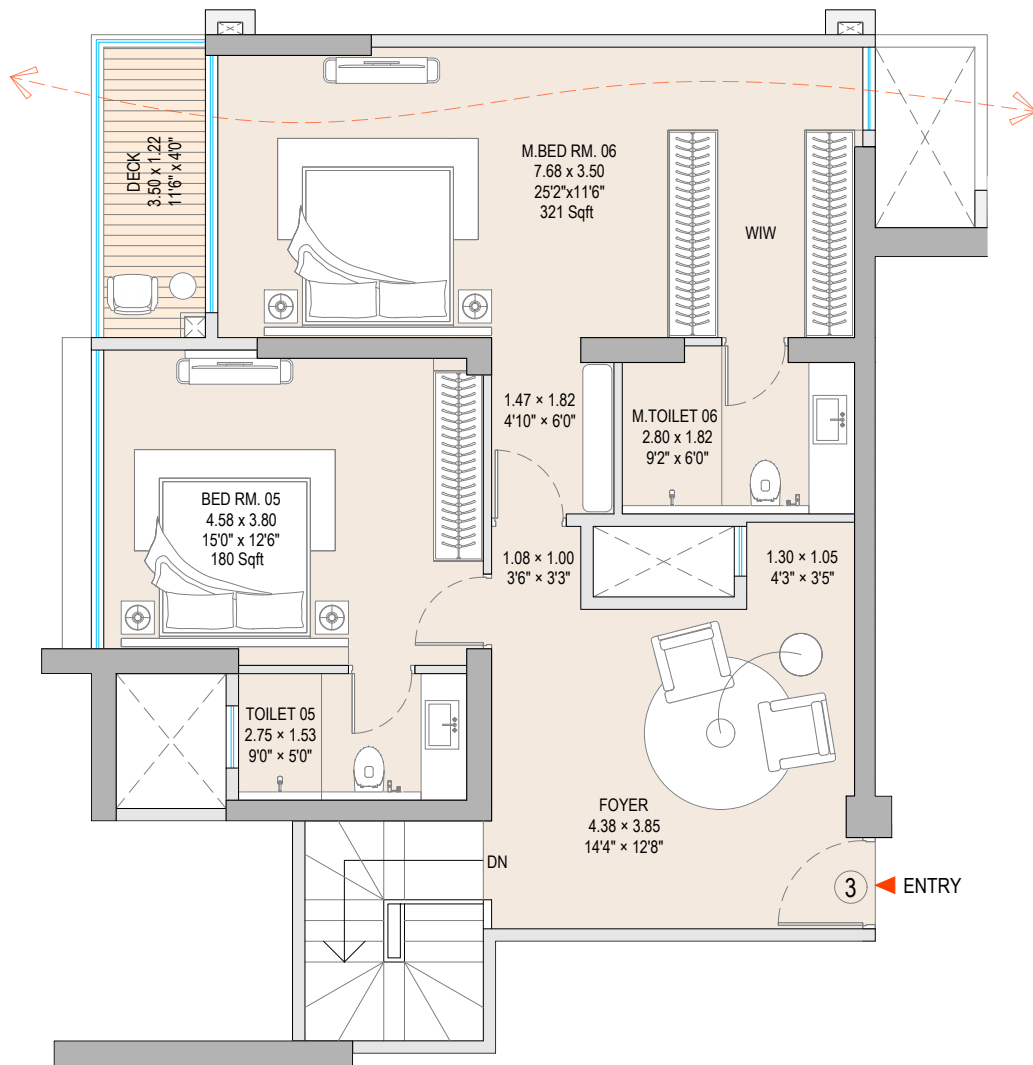
DUPLEX-UPPER LEVEL PLAN
